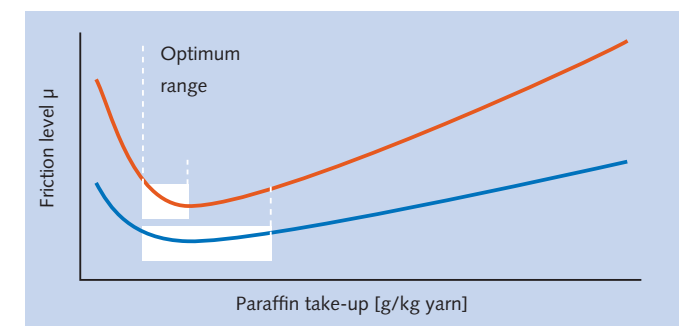
The paraffin application curve shows the ratio between the friction level and take-up by different materials such as ■ man-made fibres or ■ cotton yarns. The white area shows the optimum ratio.
